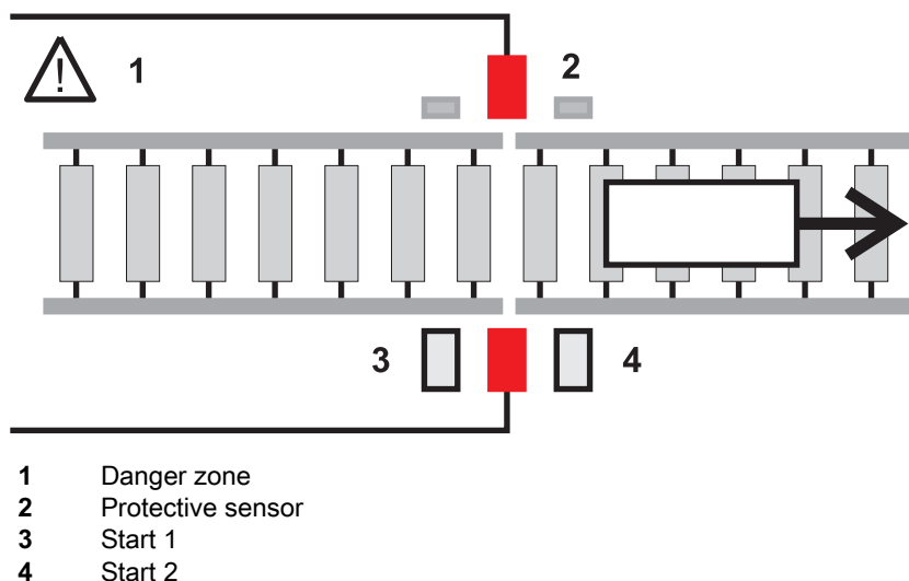
Figure 3.7: Phase 7 - End of muting
