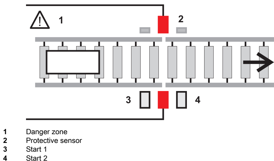
Figure 3.1: Phase 1 - Muting preparation is activated by applying the control signals. The pallet is still completely inside the danger zone.
