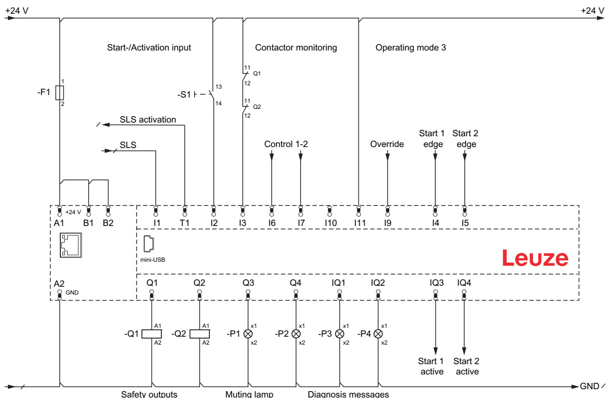
Figure 4.1: Connection example for MSI 420.TMC-03 with start/restart interlock and contactor monitoring (operating mode 3)
