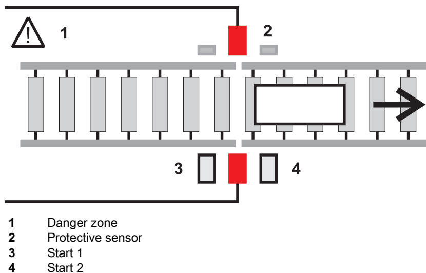
Figure 3.6: Phase 6 - Protective sensor becomes free again.
